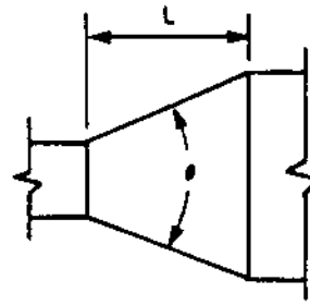
CONCENTRIC TRANSITION \theta MAX. 45° DIVERGING, 60° CONVERGING
