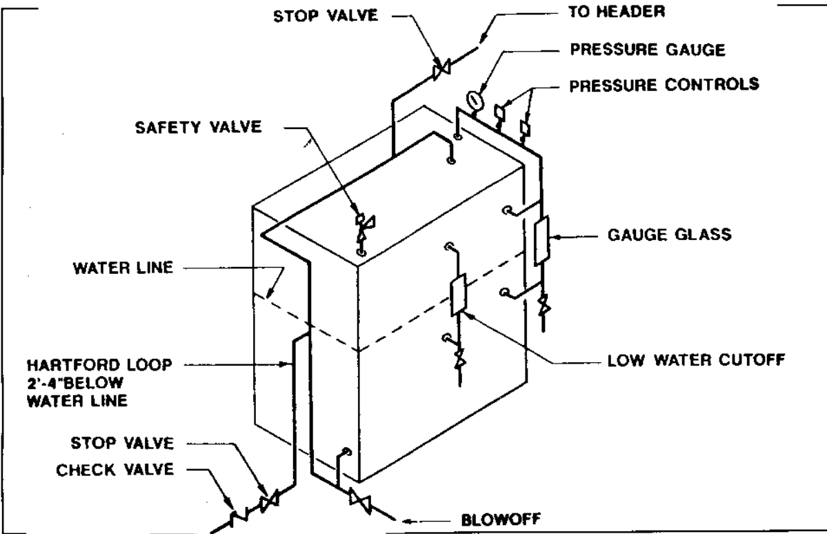
Figure 28 Boiler Connections
