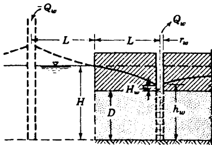
(b) ARTESIAN FLOW
