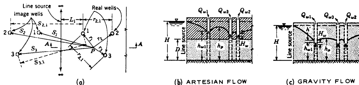
CONSTRUCTION OF THE IMAGE WELLS IS DISCUSSED IN THE TEXT OF PARAGRAPH 4-2
