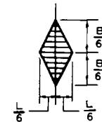
DISTRIBUTION OF BEARING PRESSURES BENEATH RECTANGULAR FOOTINGS
