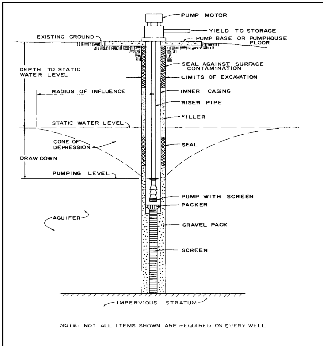
Figure 5-5. Diagrammatic Section of Gravel-packed Well.
