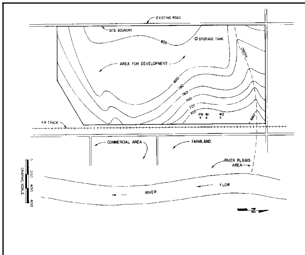
Figure B-1. Plan of Proposed Site.
