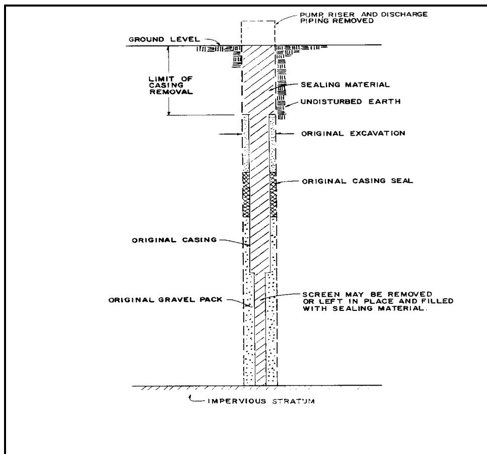
Figure 5-7. Sealed Well.
