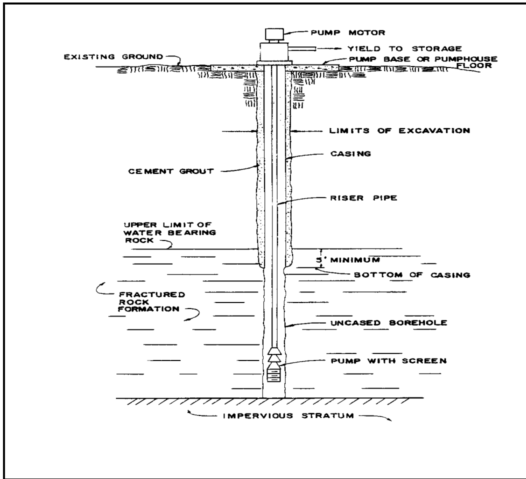
Figure 5-6. Well in Rock Formation.
