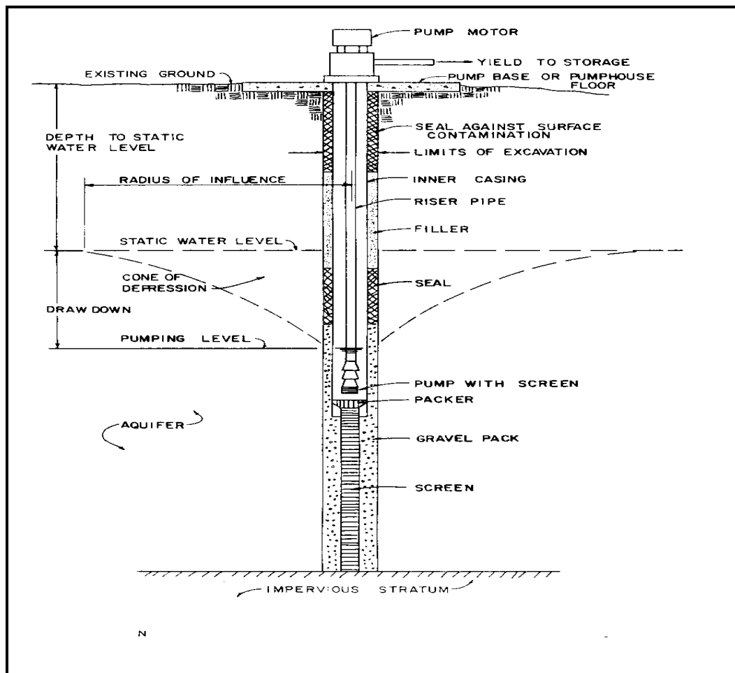
Figure 5-4. Diagram of well in artesian aquifer.
