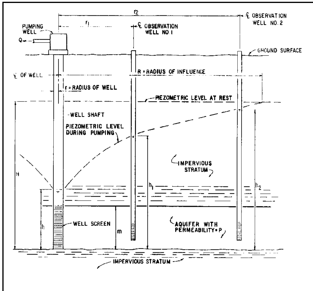
Figure 5-3. Diagram of Water Table Well (unconfined aquifer).
