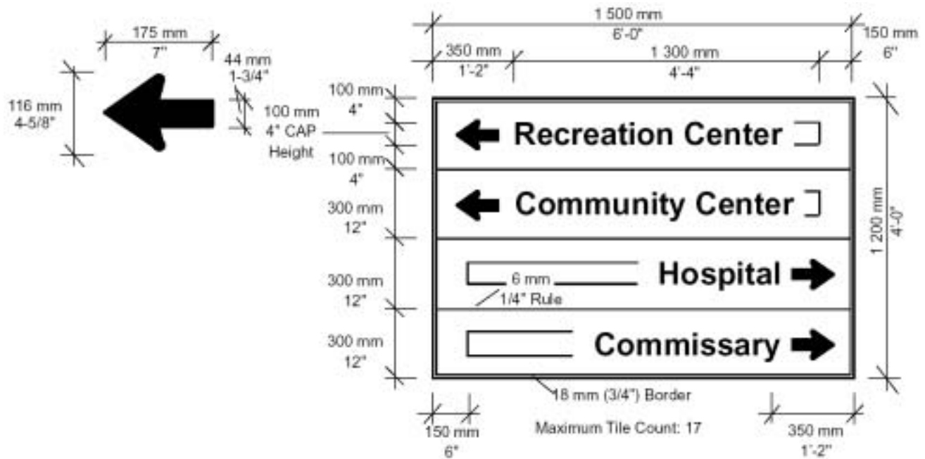
Figure 5.11. Direction Sign Type D3 Typical Panel.
