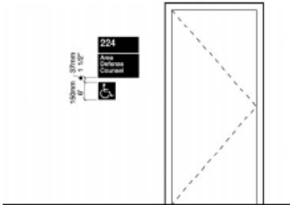
Figure 4.27. Mounting Conditions.
