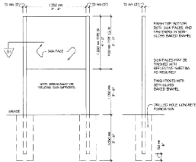
FRONT ELEVATION AND SECTION: TYPES B1, C2, H1 SCALE: 1/4"=1'-0"
