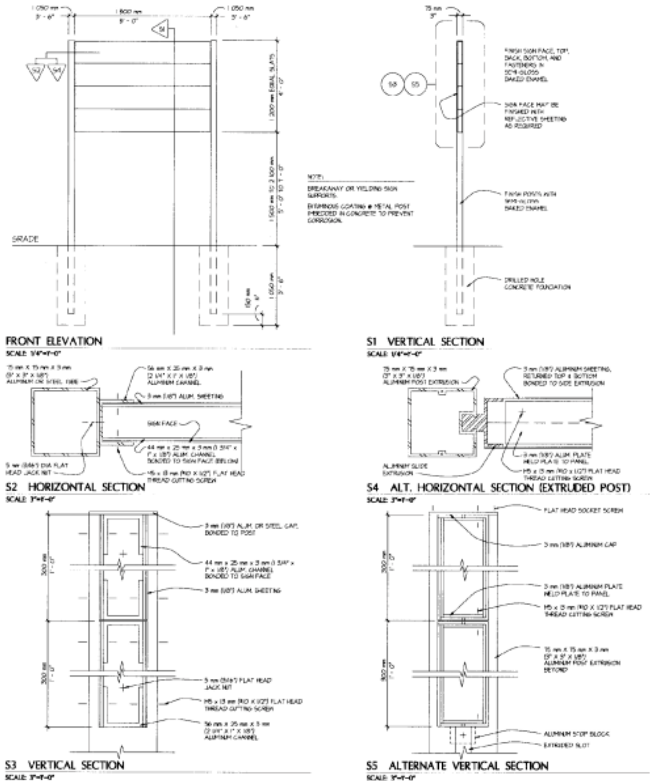
Figure 12.5. Sign Details D2.
