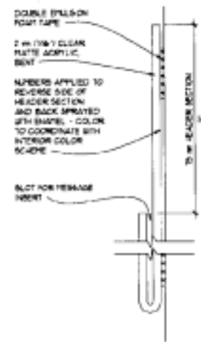
S4 VERTICAL SECTION, TYPE BB5 HALF SCALE
