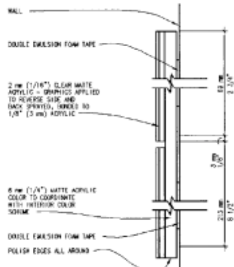
S4 ALTERNATE DETAIL, SIGN TYPE CC2, MULTIPLE
