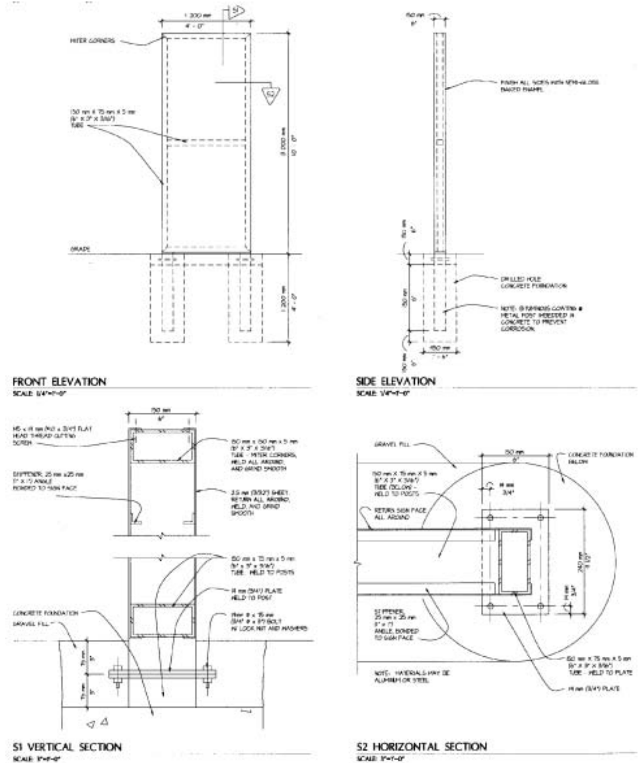
Figure 12.3. Sign Details C1.
