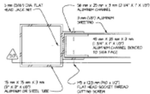
S1 HORIZONTAL SECTION SCALE: 3/4"=1'-0"
