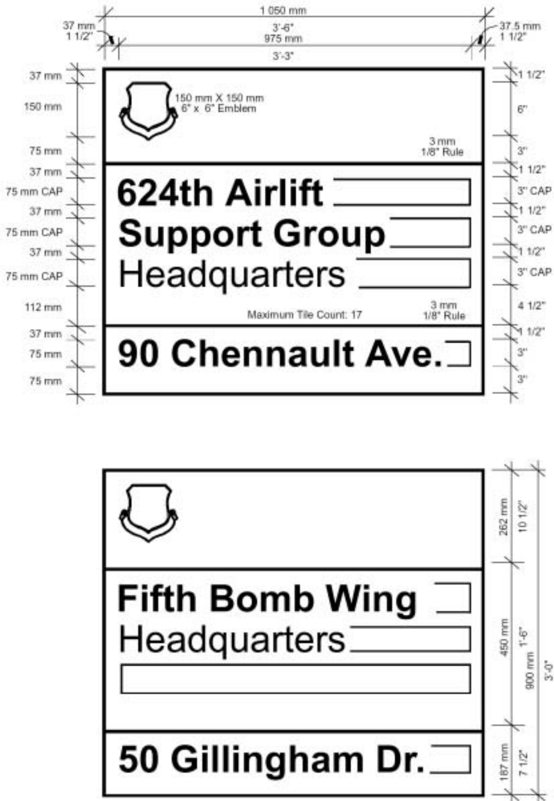
Figure 4.18. Military Identification Sign Type B2 Layouts.
