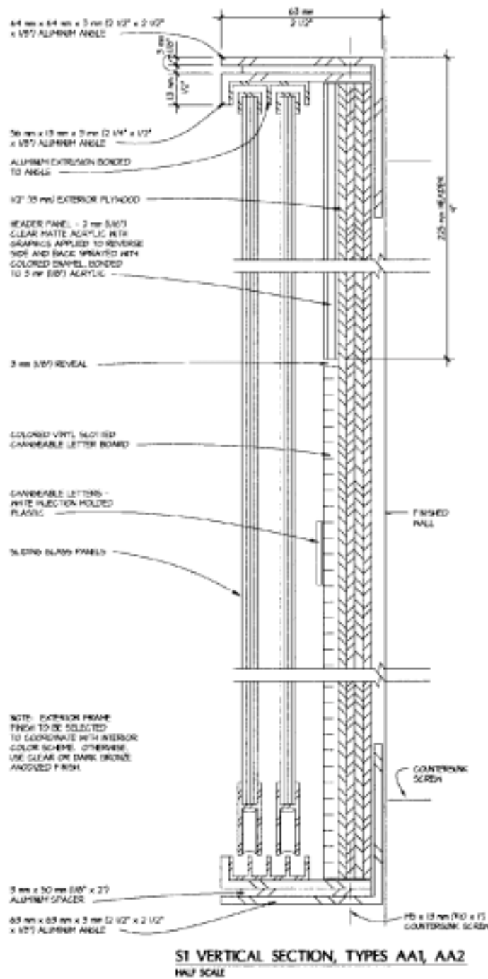
Figure 12.13. Sign Details AA1, AA2, AA3.
