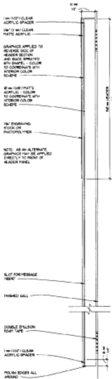
S1 VERTICAL SECTION, TYPE BB1 HALF FULL SCALE
