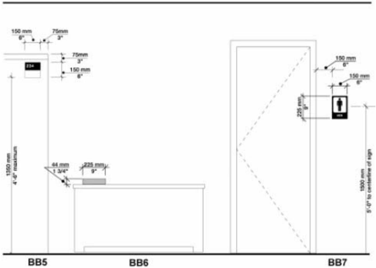
Figure 11.11. Placement of Identification Signs Types BB5, BB6 and BB7.
