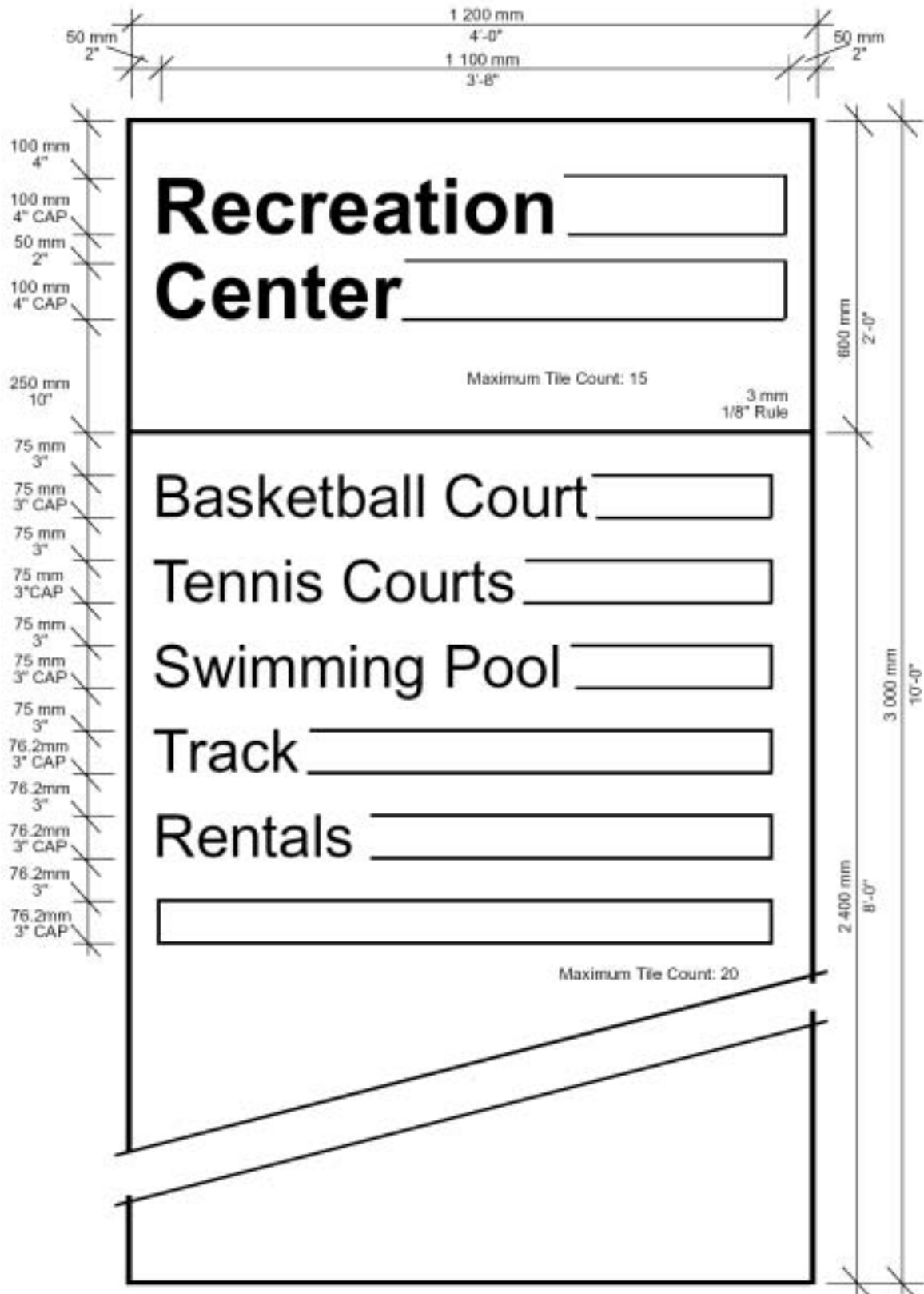
Figure 4.36. Centralized Facilities Sign Type C1 Layout B.
