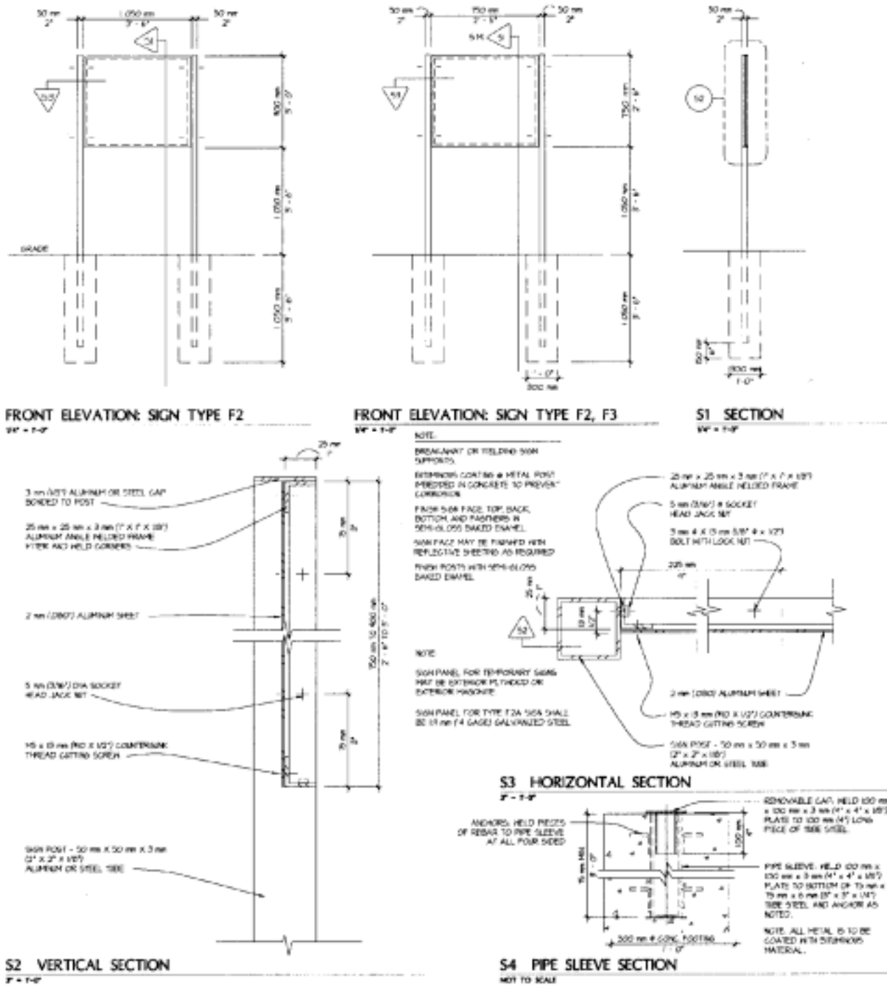
Figure 12.8. Sign Details F2 and F3.
