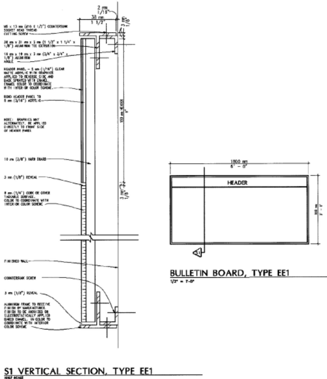
Figure 12.20. Sign Details EE1.
