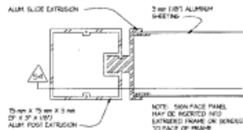
S2 ALT. HORIZONTAL SECTION (EXTRUDED POST) SCALE: 3/4"=1'-0"
