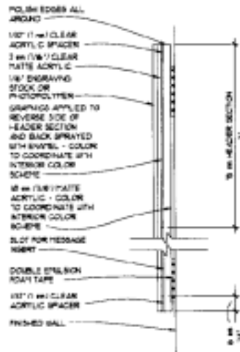
Figure 12.15. Sign Details, BB1, BB2, BB3, BB4 and BB5.
