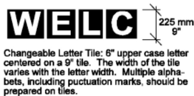
Figure 7.6. Changeable Letter Tile Dimensions.
