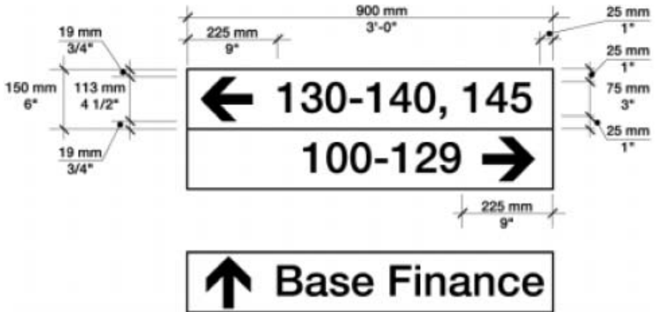
Figure 11.16. Direction Sign Type CC1 Layout.
