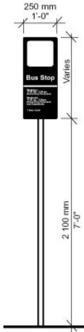
Figure 4.47. Bus Route Sign Type C6 Placement.
