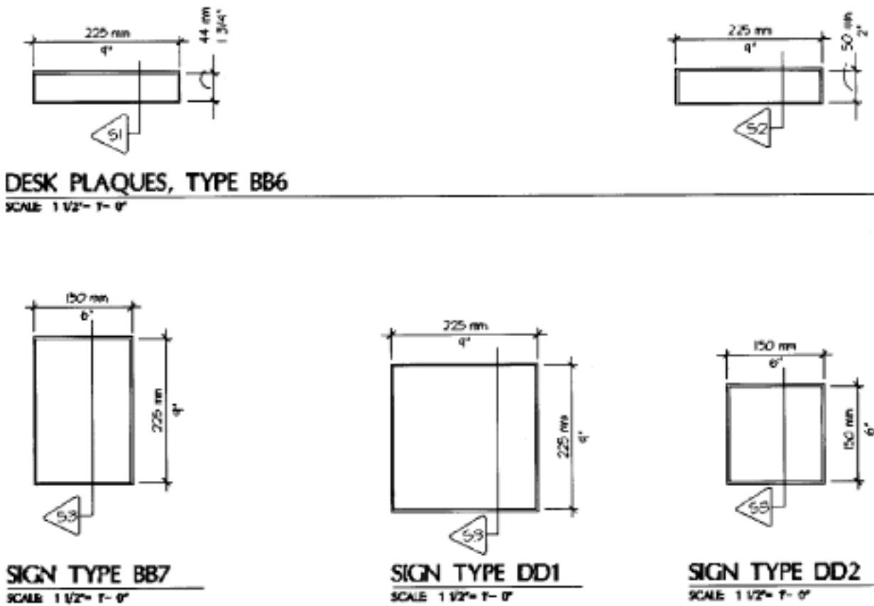
Figure 12.16. Sign Details BB6, BB7, DD1 and DD2.
