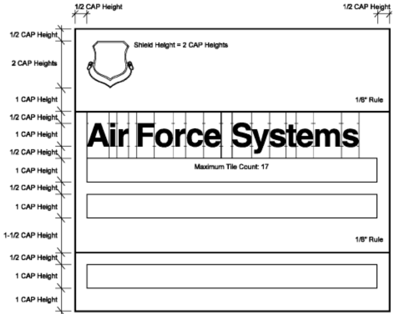
Figure 2.7. Sign Grid.
