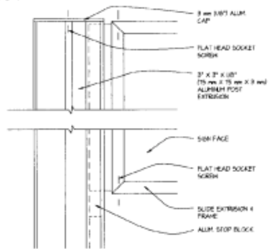
S4 ALT. VERTICAL SECTION SCALE: 3/4"=1'-0"
