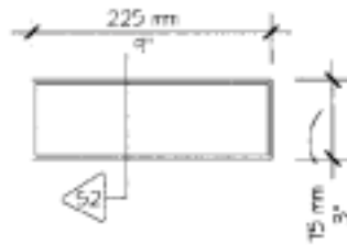
Figure 12.14. Sign Details BB1, BB2, BB3, BB4, BB5.
