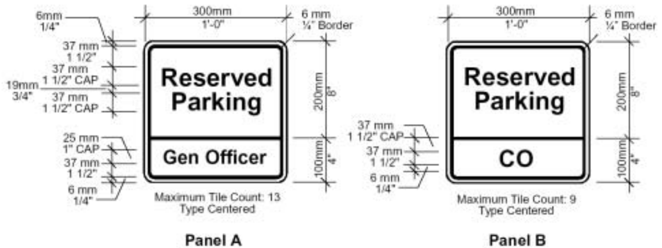
Figure 6.14. Parking Regulation Sign Type E2.
