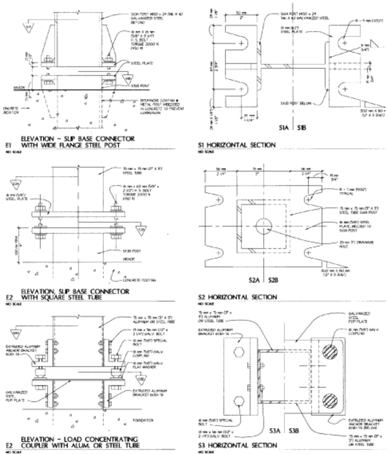
Figure 12.10. Sign Details.
