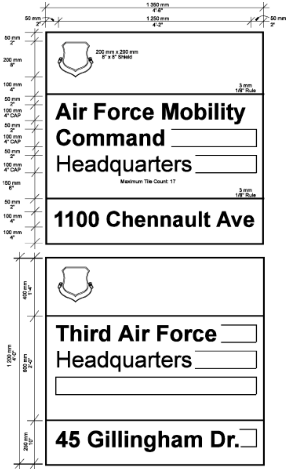
Figure 4.16. Military Identification Sign Type B1 Layouts.
