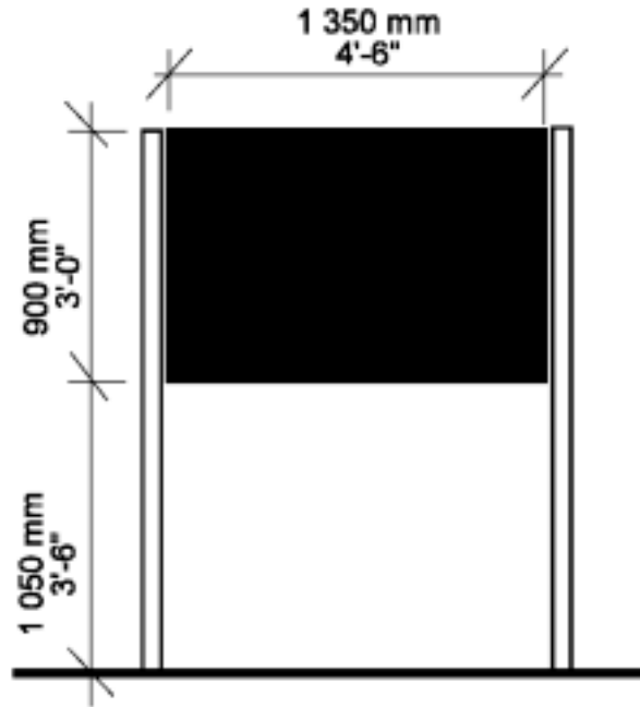
Figure 4.29. Community Facilities Type C2.
